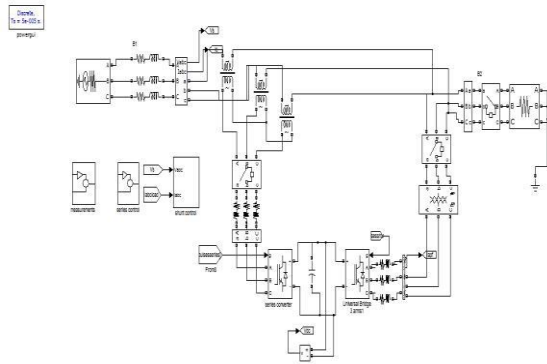
Fig.4. MatLab/Simulink diagram of modified iUPQC
