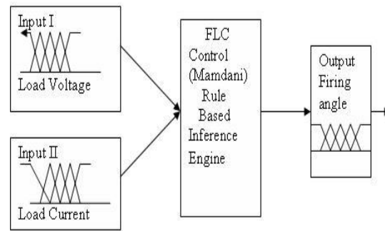
Fig.2. Structure of fuzzy logic controller
