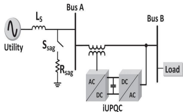
Fig.3. iUPQC experimental scheme
