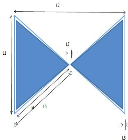
Figure 2: Geometry of the proposed antenna
