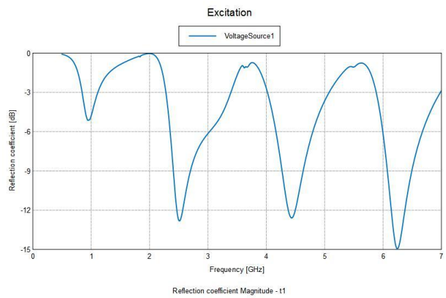
Figure 3: Return loss characteristics of proposed antenna
