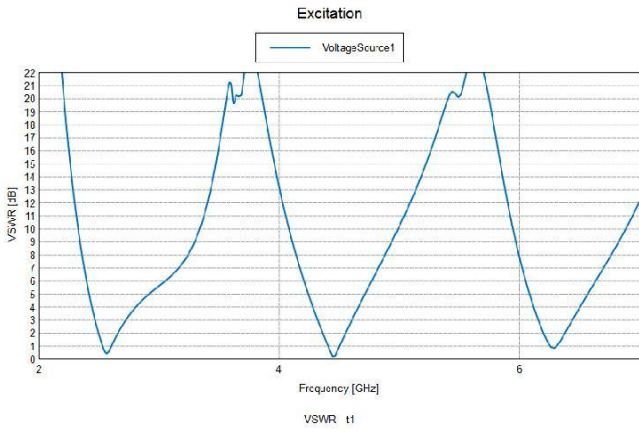
Figure 5:VSWR characteristics of proposed antenna
