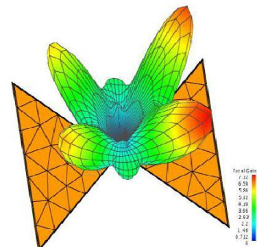
(e) Far field pattern at 6.2GHz
