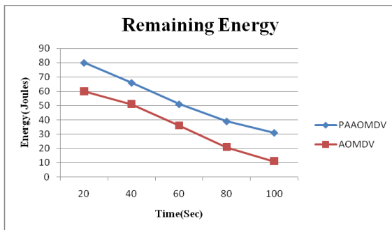
Figure 4 Remaining energy comparisons
