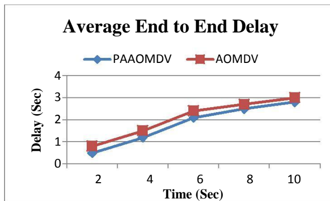
Figure 2 End to End delay comparison
