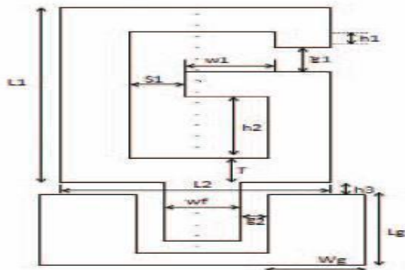
Figure 3: Geometry of the G-shaped Antenna[7]
