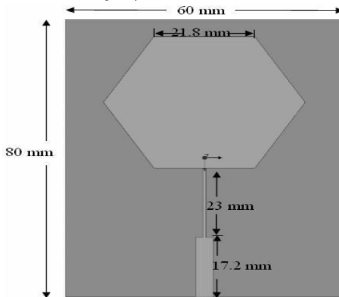
Figure 5:Geometry of the hexagonal line fed antenna[9]
