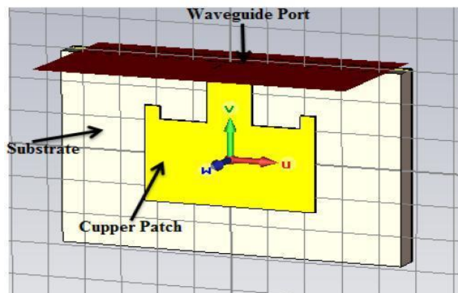
Figure 2: Wideband inset fed Antenna Geometry [6]
