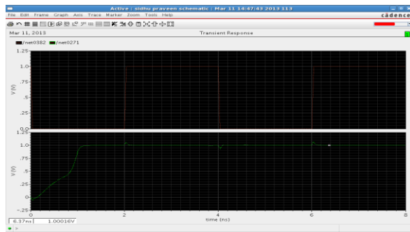
Fig 3.4 Input of D and Output of Q in CPSIPFF
