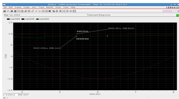
Fig 3.5 output of CPSIPFF existing and modified
