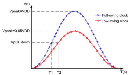
Fig.2.2. Delay between the low and full-swing resonant clock signals to reach V_{pull\_down}
