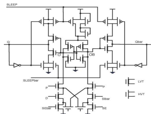
Figure 3 Double Edge Triggered State Retention Scan Flip-Flop(DETSRSFF)
