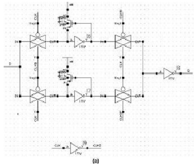
Figure 2 a) Gated double edge trigger flip-flop
