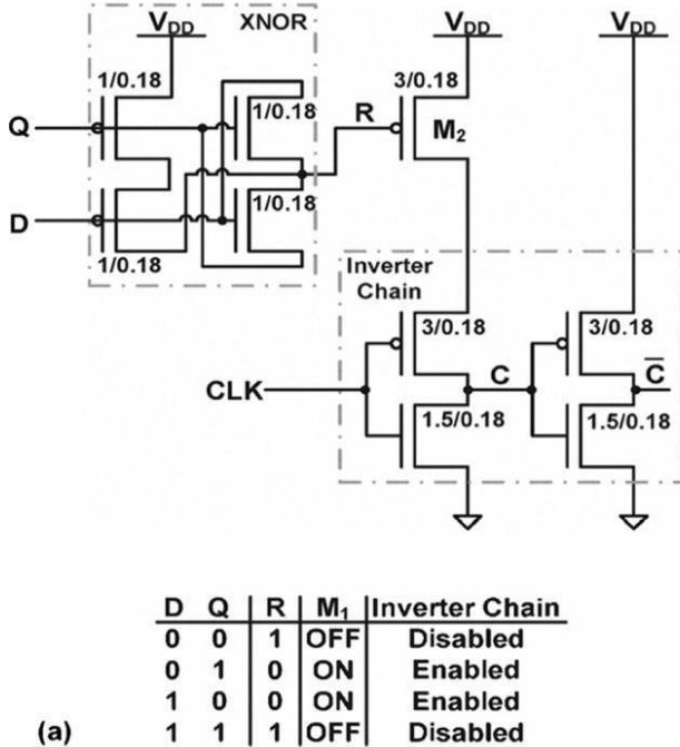
Figure 4 Clock Gating and Internal Clocking Circuitry
