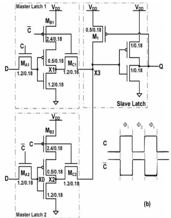
Figure 5 Flip-Flop Circuitry
