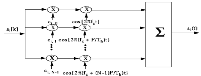
Fig. 1. Spreading in MC-CDMA
