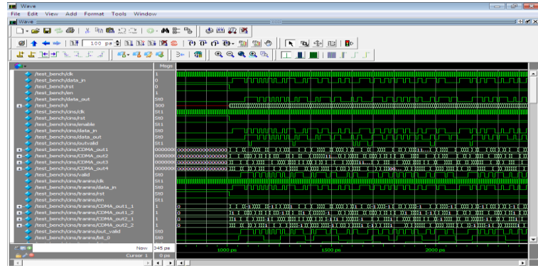
Fig 5. Simulated output
