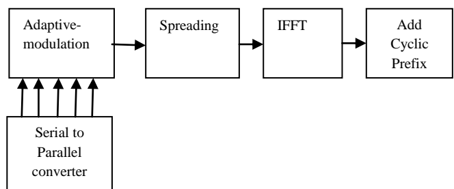
Fig 2.MC-CDMA Transmitter side block diagram
