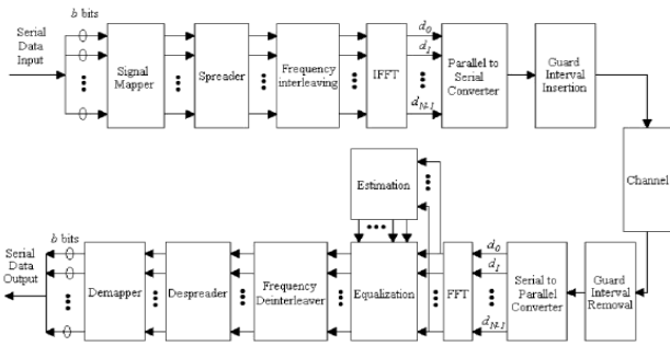
Fig 4. MC-CDMA Transceiver design block diagram
